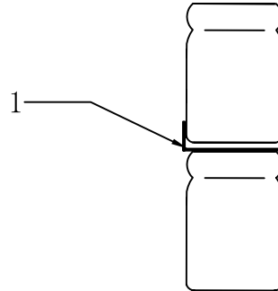
Weld Schematic Drawing
