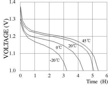
DISCHARGE CURVE AT VARIOUS TEMPERATURES (32mA)
