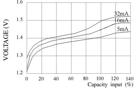
TYPICAL CHARGE CURVE AT VARIOUS CURRENTS
